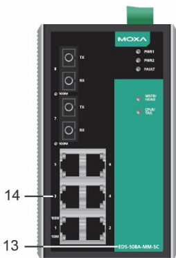
EDS-508A-MM-SC Front Panel View
