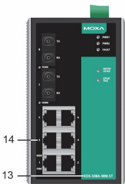
EDS-508A-MM-ST Front Panel View
