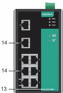
EDS-508A Front Panel View
